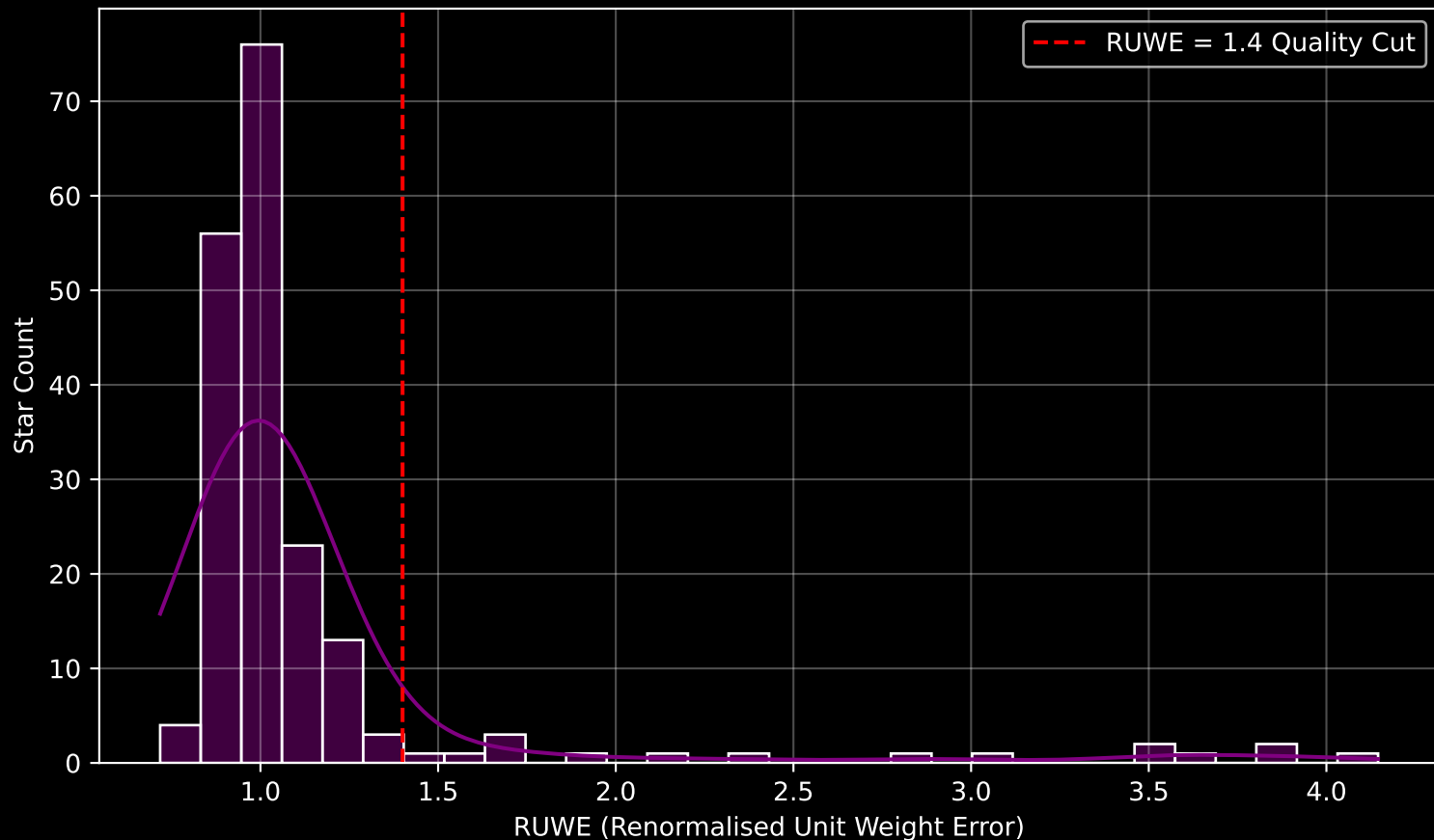
GAPOGEE DR17 Field [K2_C7_020-17_btx] RUWE Distribution (n= 191)
