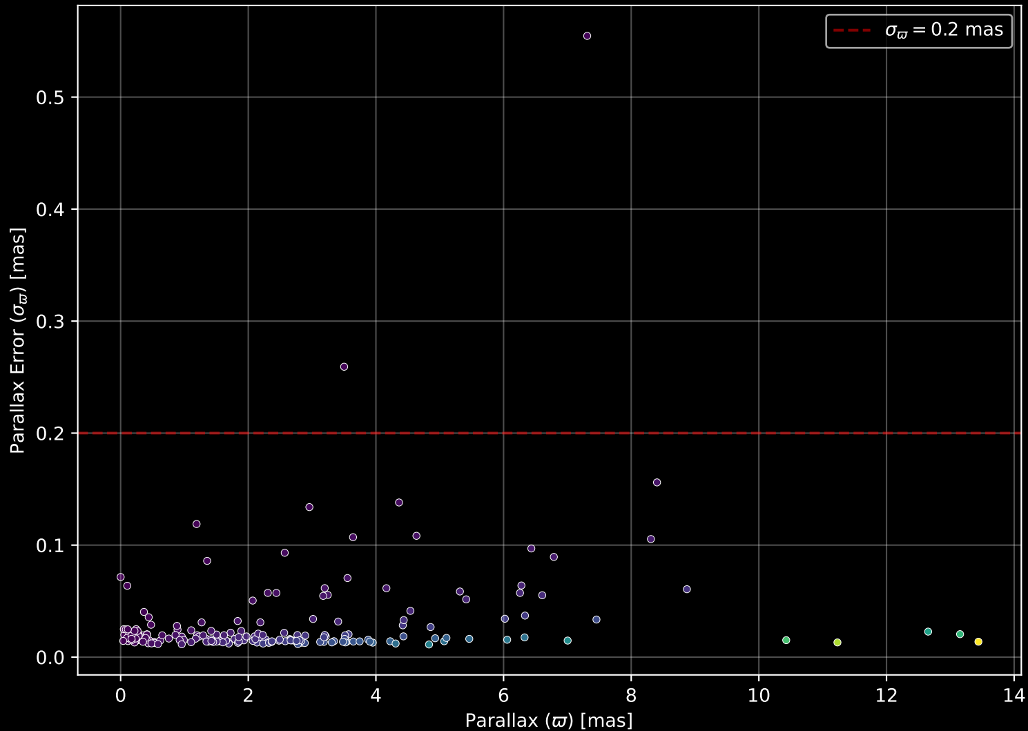
APOGEE DR17 Field: [K2_C7_020-17_btx] Parallax Quality (n= 196)
