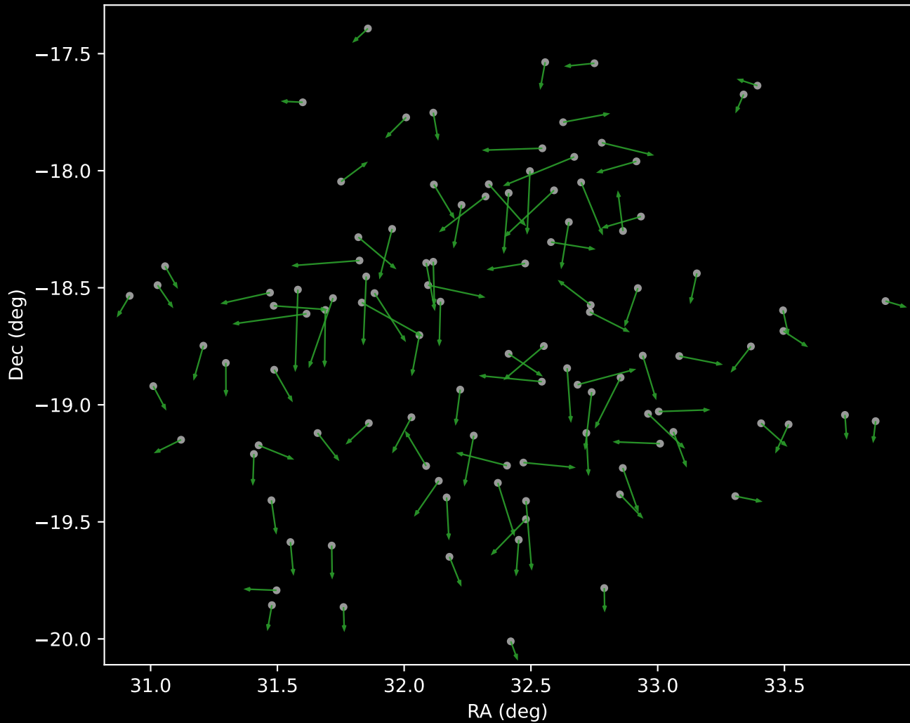
APOGEE DR17 Cluster 4 Proper Motion Vectors (n=106)
