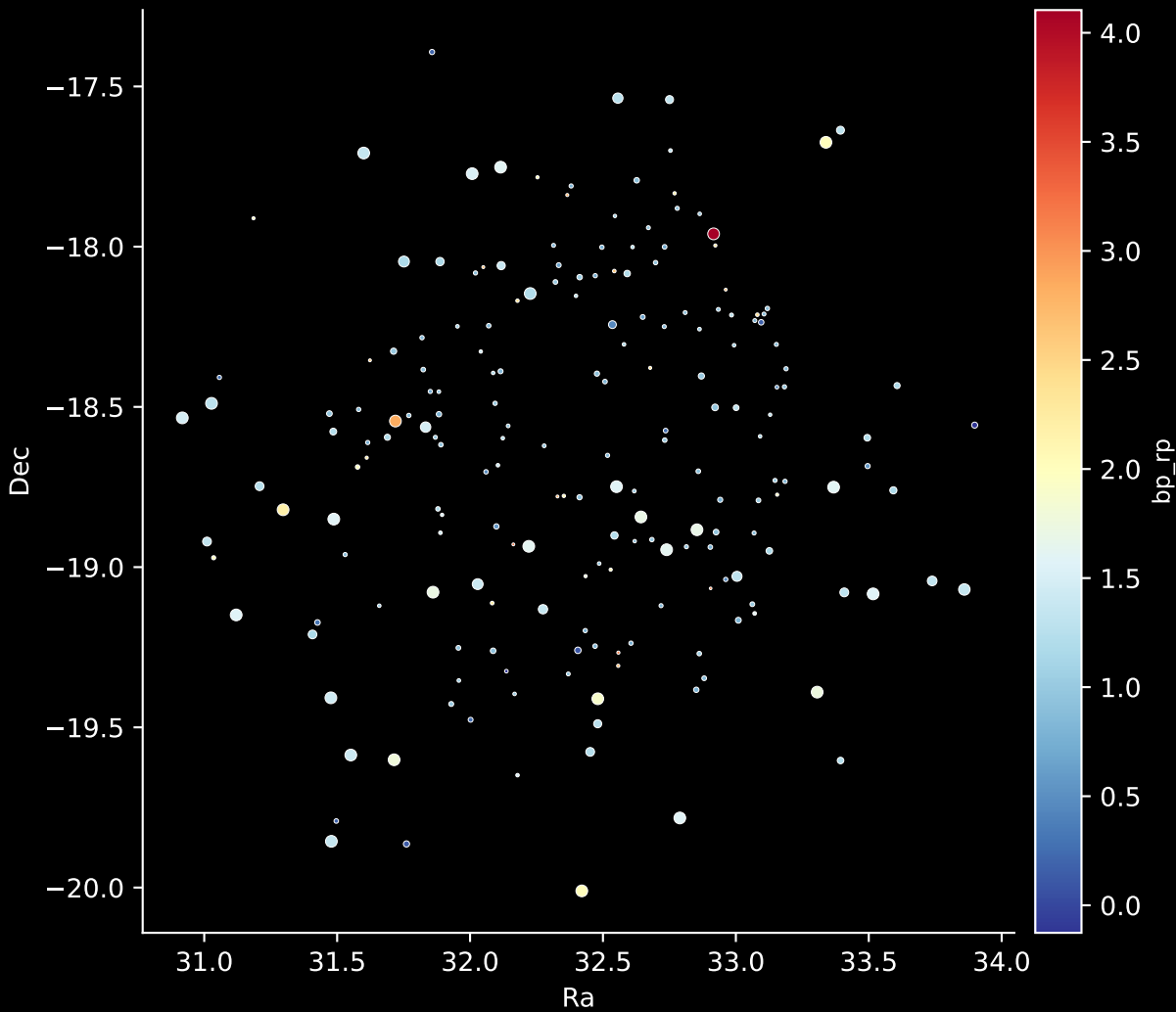
APOGEE DR17 Field: [K2_C7_020-17_btx] Stars: 196
