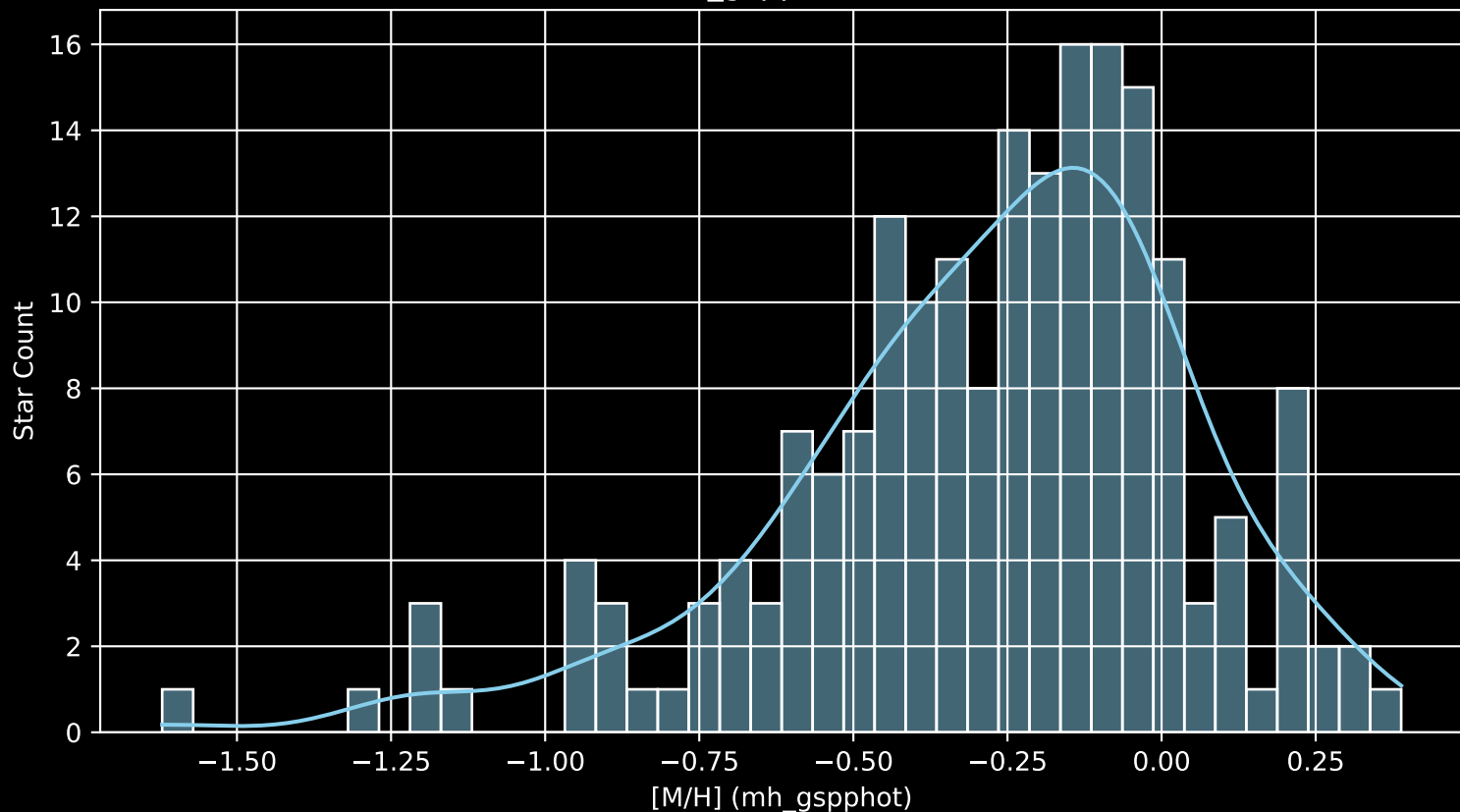
APOGEE DR17 Field: [K2_C7_020-17_btx [M/H] (mh_gspphot) (n= 193)
