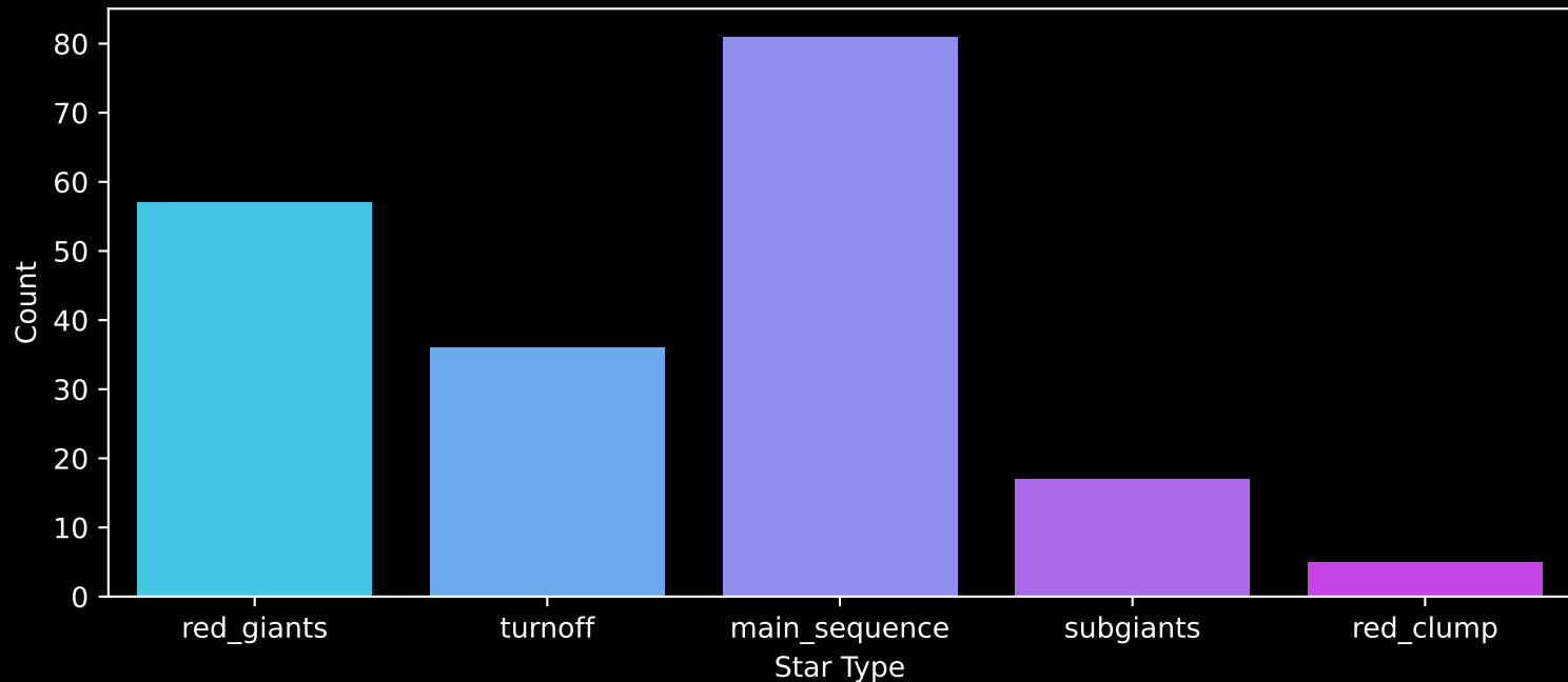
APOGEE DR17 Field: [K2_C7_020-17_btx] Count plot of Star Type
