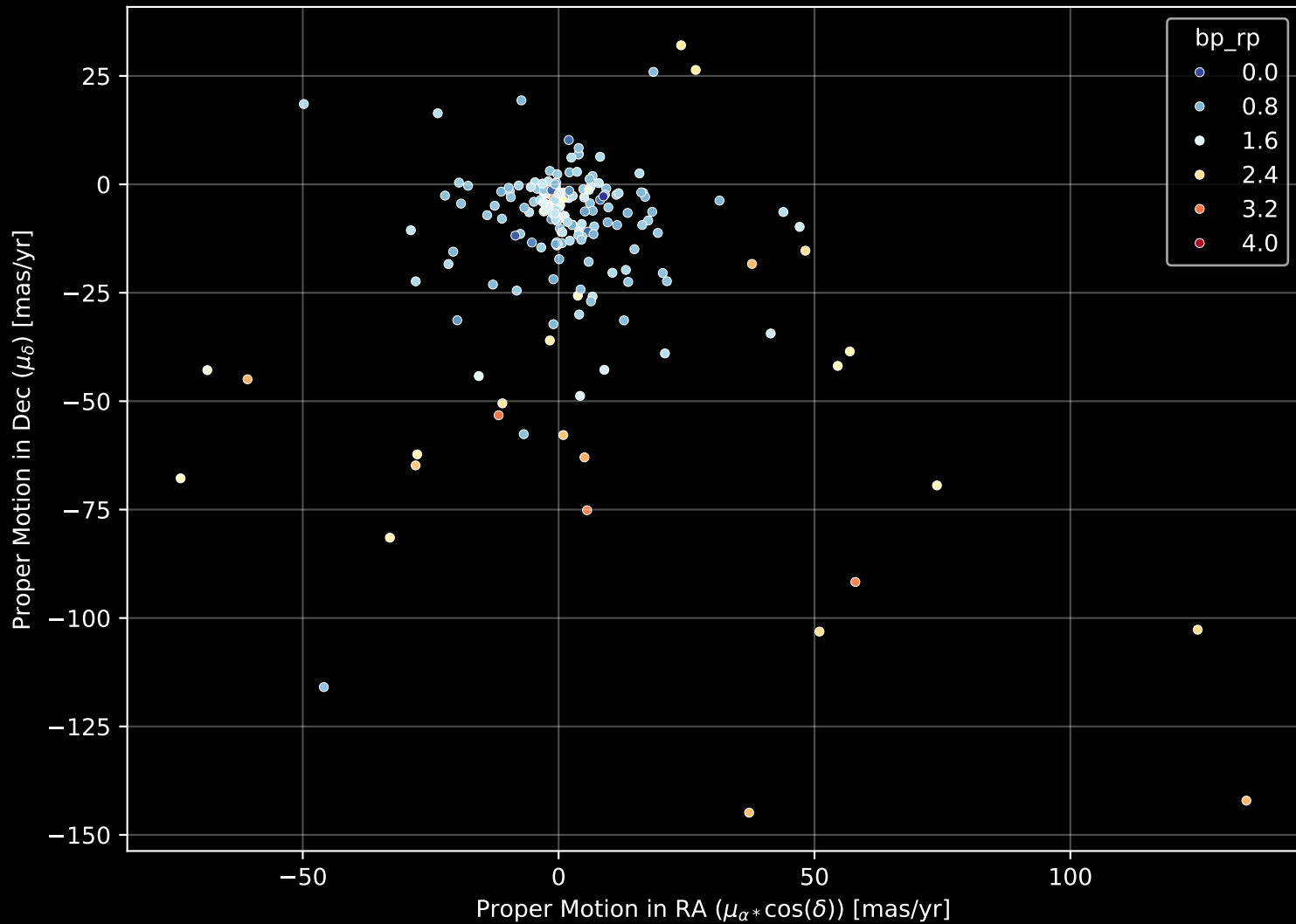
APOGEE DR17 Field: [K2_C7_020-17_btx] Proper Motion Diagram (n= 196)
